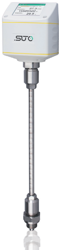
S401/S421
